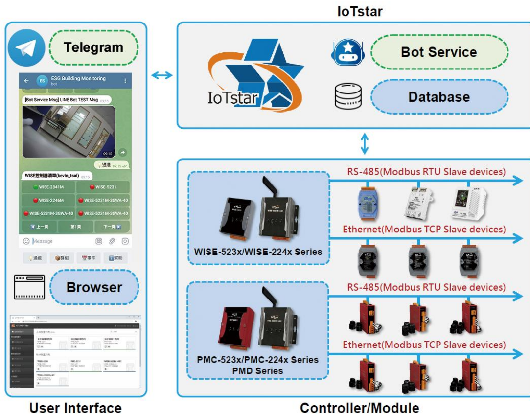
Figure 1-2: System Architecture of IoTstar 2025 Bot Service (Telegram)
