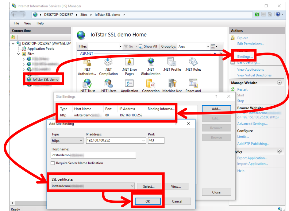
Figure 2-9: Enable the HTTPS connection of the IoTstar website
