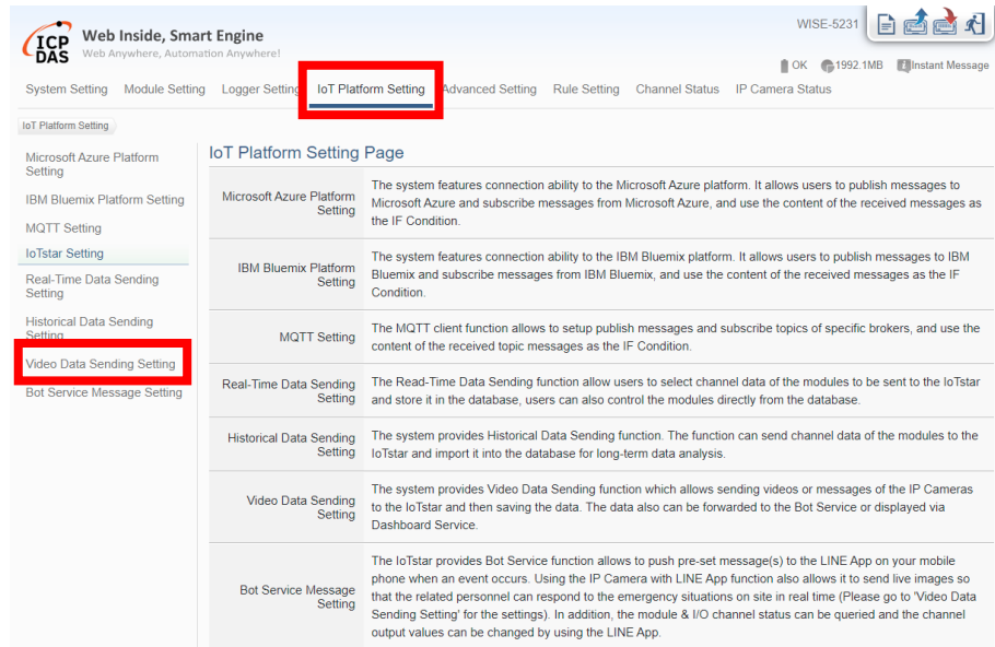
Figure 2-15: WISE Web Site - Bot Service Forward Setting Page (1)
